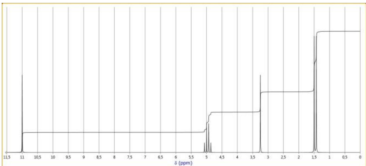
Spectre 1
