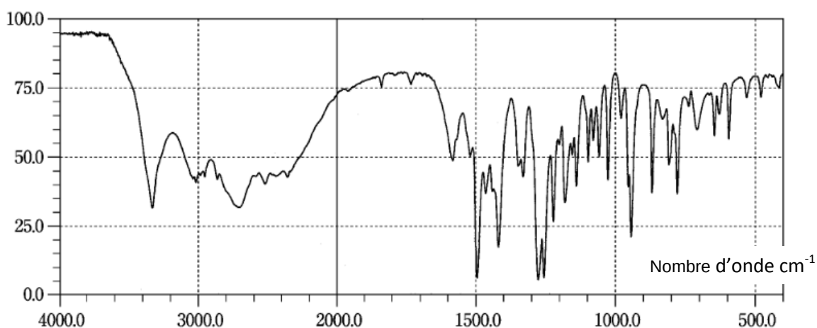
Spectre IR
