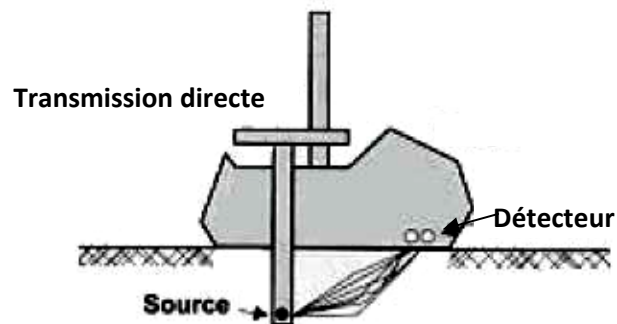
Transmission directe
