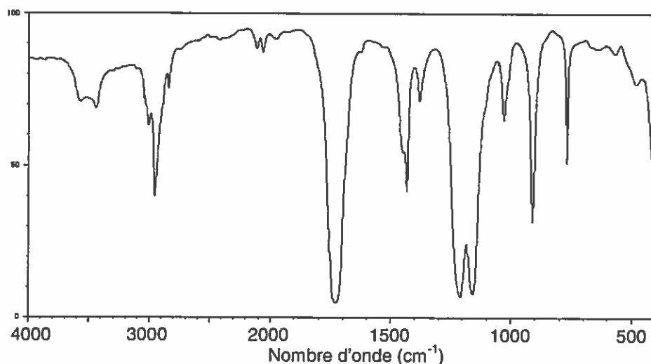
Spectre IR 2
